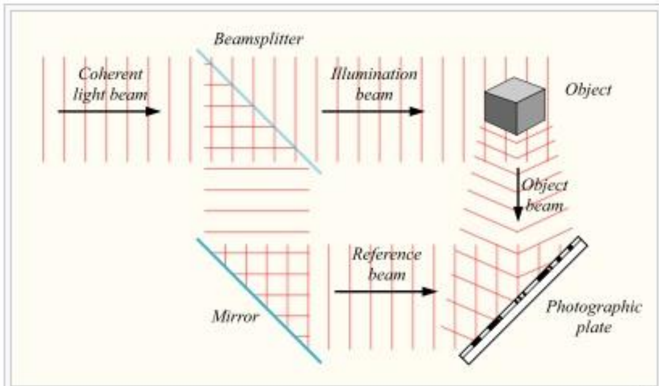
Recording a hologram
